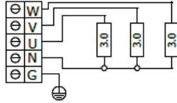
ARI3-90NS-WL 9,0 kW
